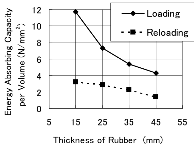
Fig.8 Energy Absorbing Capacities per Volume
