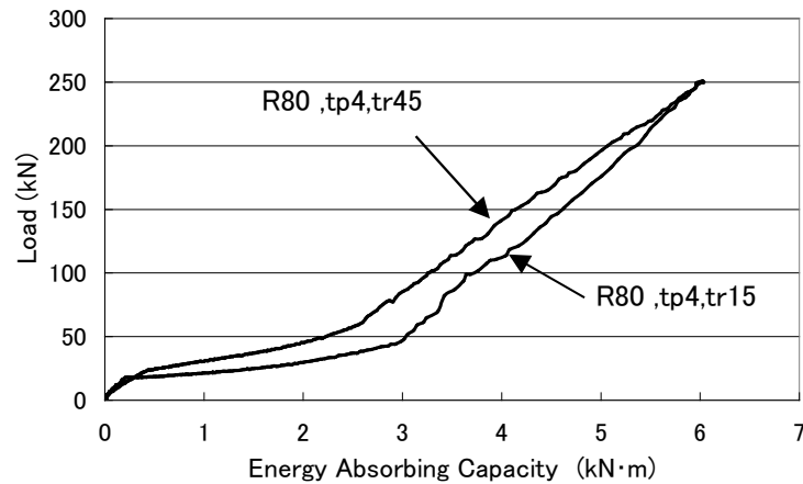
Fig. 10 Comparison of Collision Force
