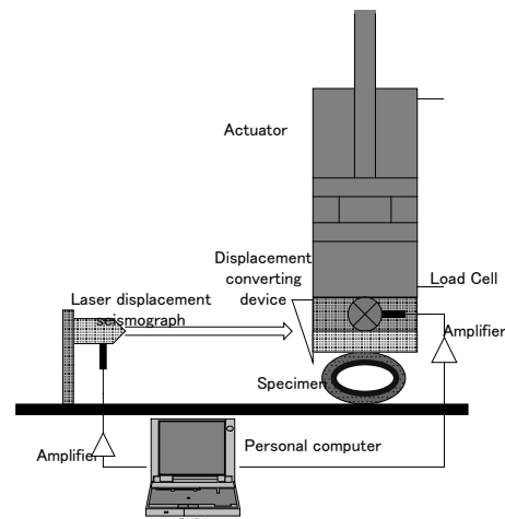
Fig.2. Outline of Loading Test Equipment
