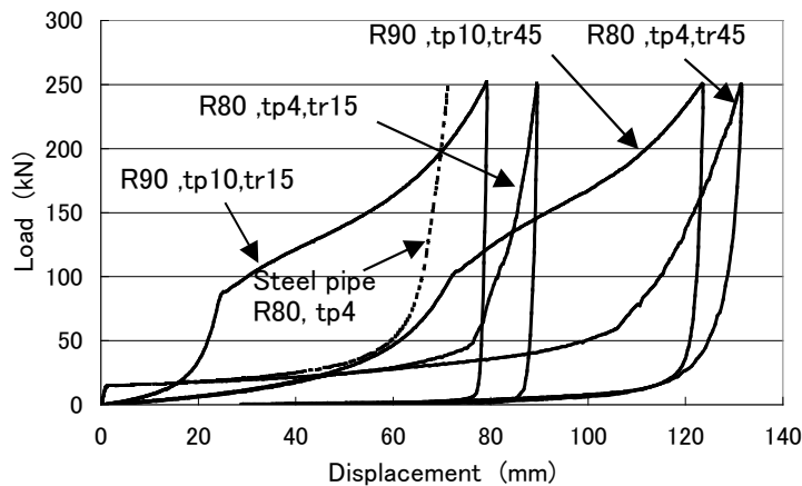
Fig. 3. Load-Displacement Characteristics of Shock Absorbers
