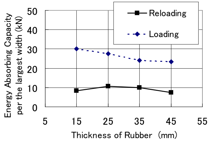
Fig.7 Energy Absorbing Capacity per the Largest Width
