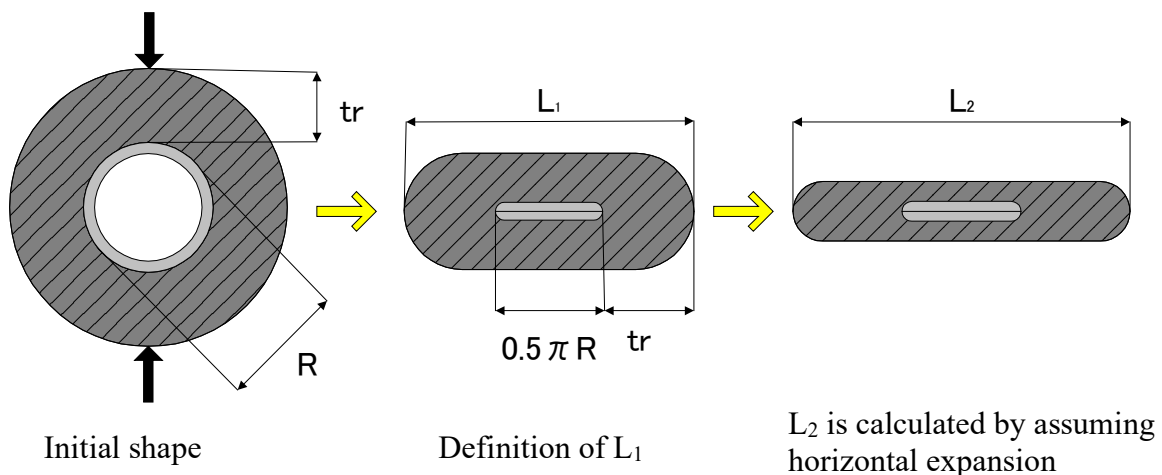
Fig.6. Estimating Horizontal Strain of Shock Absorbers
