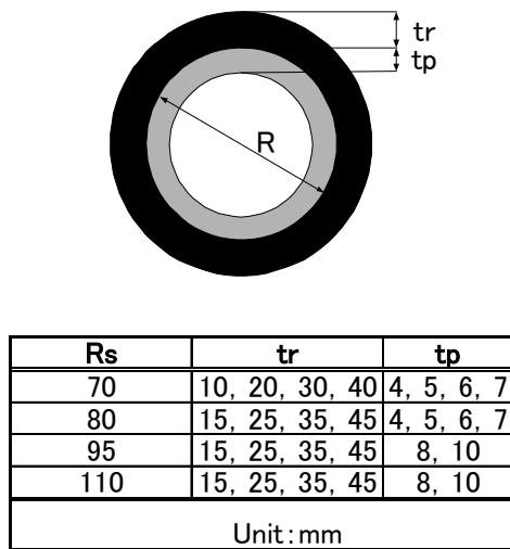
Fig. 1. Sizes and Shape of Test Specimens
