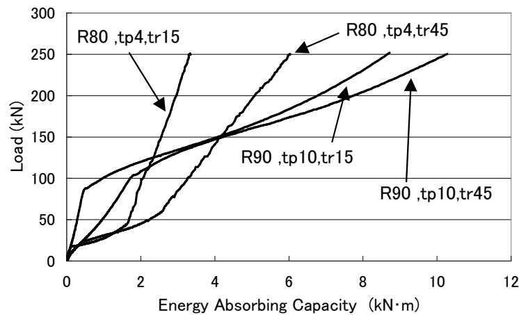
Fig. 5. Load-Energy Absorbing Capacity Characteristics of Shock Absorbers
