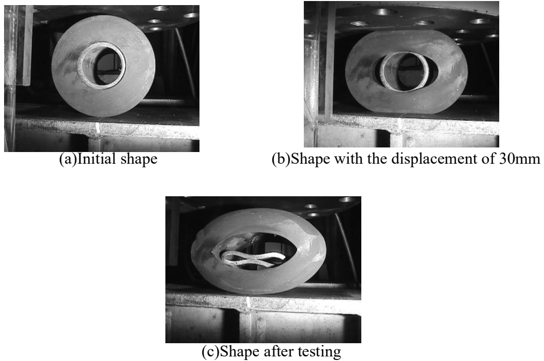
Fig. 4. Deformation of a Specimen (R80mm, tp6mm, tr40mm)
